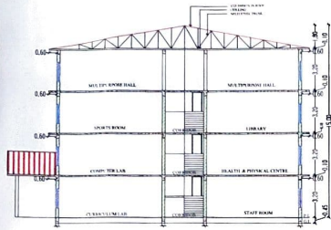
SECTION AT Y-Y
